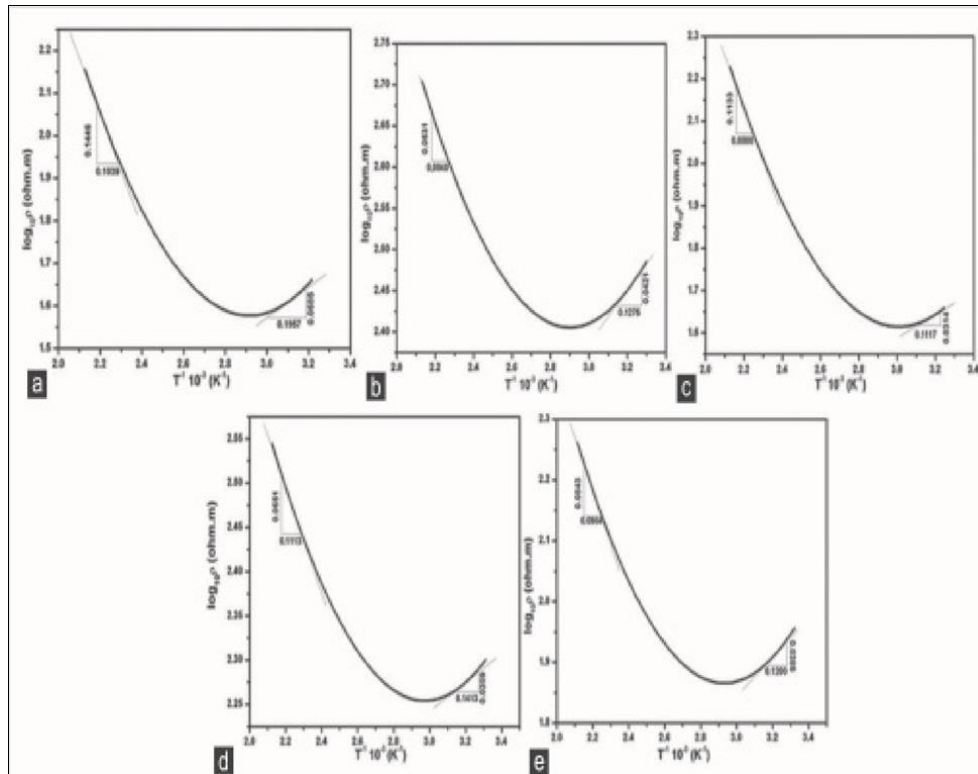
Fig 9: (a) Graph between \text{Log}_{10}\rho Versus T^{-1} for A1, (b) graph between \text{Log}_{10}\rho Versus T^{-1} for A2, (c) Graph between \text{Log}_{10}\rho Versus T^{-1} for A3, (d) graph between \text{Log}_{10}\rho Versus T^{-1} for A4, (e) graph between \text{Log}_{10}\rho Versus T^{-1} for A5
