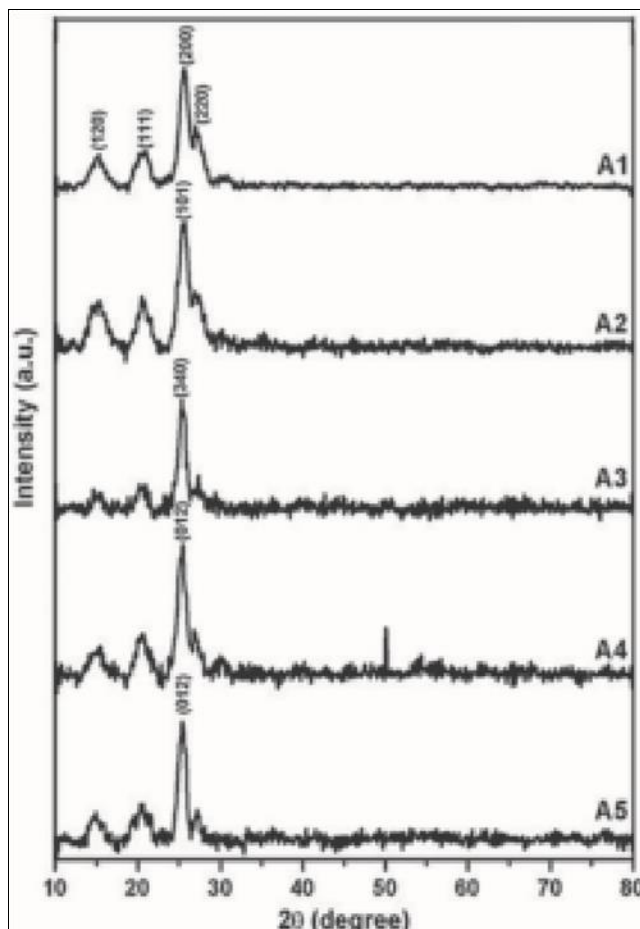
Fig 2: X-Ray Diffraction Pattern of A1-A5 Nano composites
