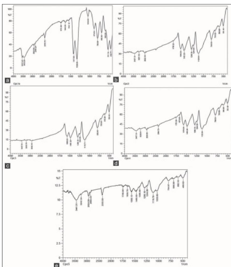
Fig 4: (a) Fourier Transform Infrared (FT-IR) Spectrum of A1, (b) FT-IR Spectrum of A2, (c) FT-IR Spectrum of A3, (d) FT-IR Spectrum of A4, (e) FT-IR Spectrum of A5
