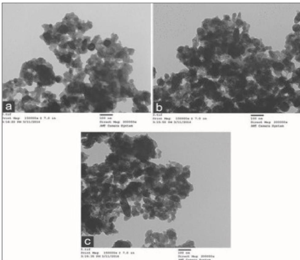
Fig 7: (a-c) Transmission Electron Microscopy Image of A3 Nanocomposite
