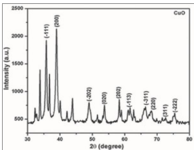
Fig 1: X-ray Diffraction Pattern of Pure Copper Oxide Sample
