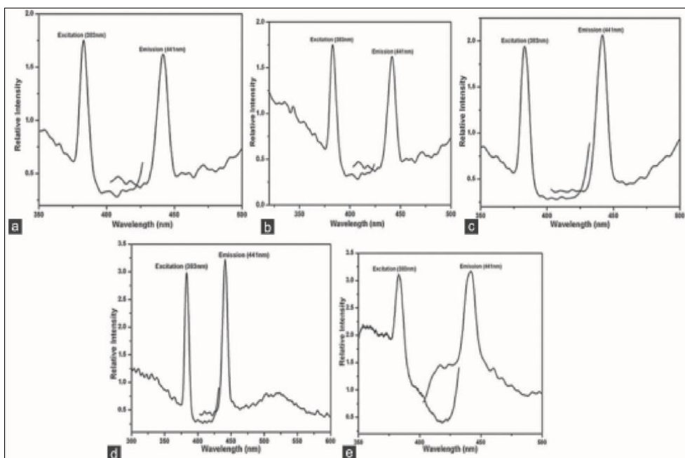
Fig 8: (a) Photoluminescence (PL) Spectrum of A1 Nanocomposite, (b) PL Spectrum of A2 Nanocomposite, (c) PL Spectrum of A3 Nanocomposite, (d) PL Spectrum of A4 Nanocomposite, (e) PL Spectrum of A5 Nanocomposite
