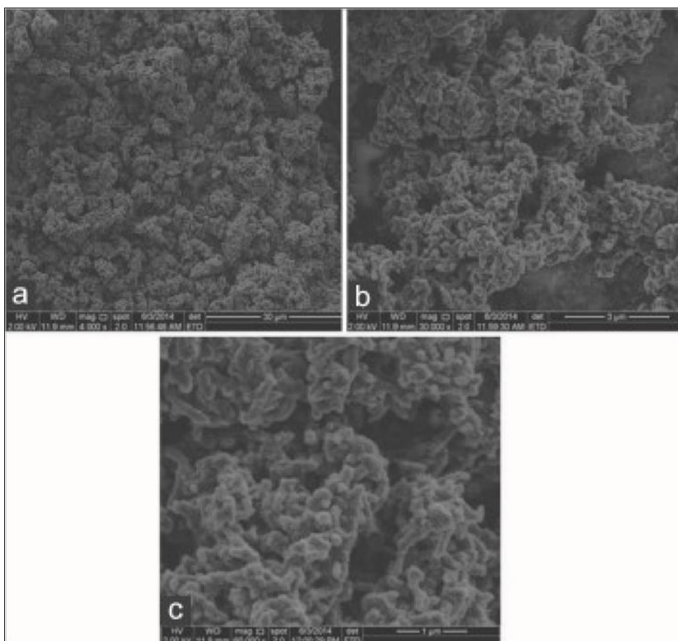
Fig 6: (a-c) Scanning Electron Microscopy Image of A3 Nanocomposite
